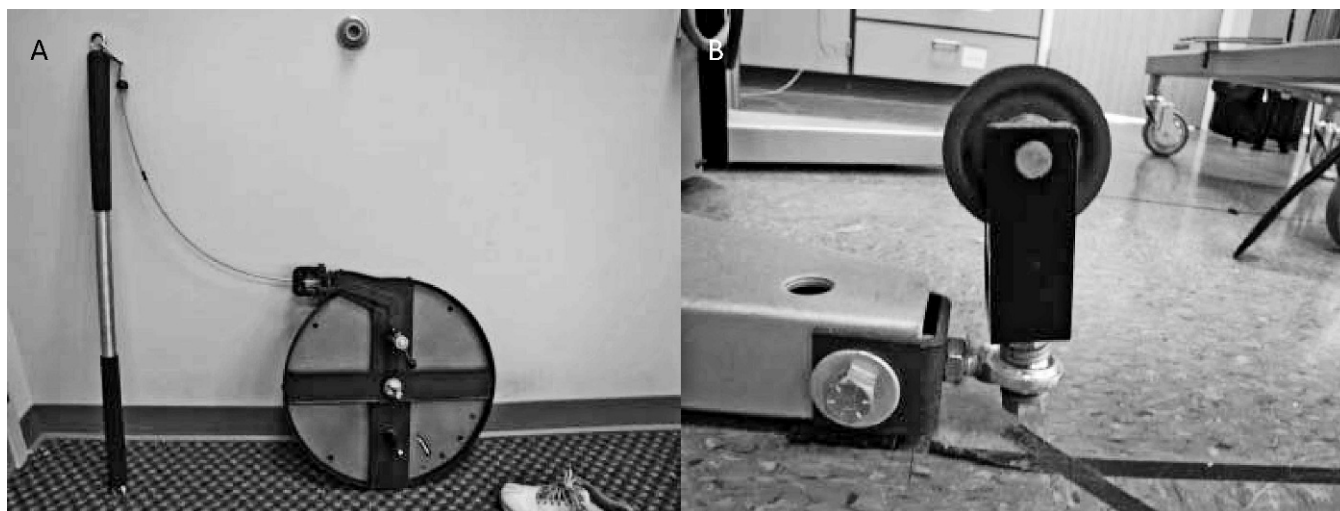
Figure 3. The PrimusRS 3-dimensional motion system (BTE Technologies, Inc, Hanover, MD) consists of a rotating head attaching a 9-ft (2.75-m) cable through a grounded pulley to a 36-in (91.44-cm), 1.9-lb (0.86-kg) dowel rod to allow for linear displacement. A, BTE PrimusRS 3-dimensional motion system. B, Grounded pulley.
