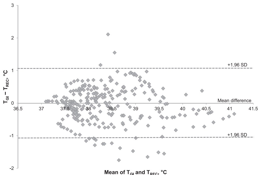
Figure 3. Bland-Altman plot depicting the differences between gastrointestinal temperature ( T_{GI} ) and rectal temperature ( T_{REC} ) observed during the 20-minute posttrace passive rest.
